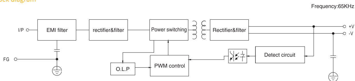
Block diagram
