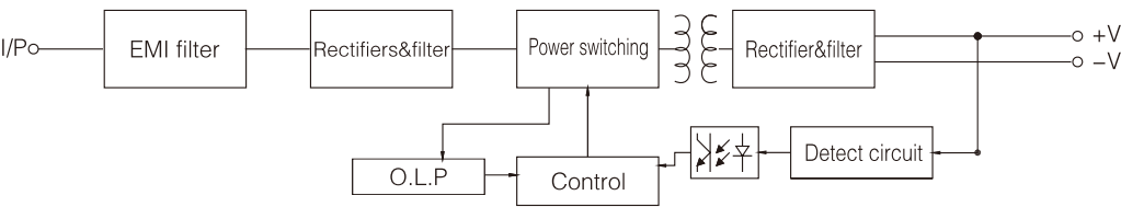
Block diagram
