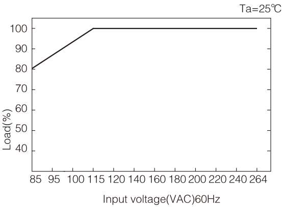
Static characteristic(24V)
