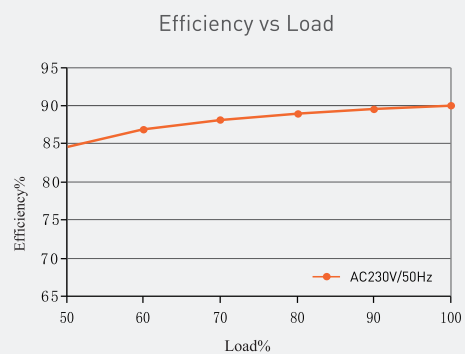
SLIM-24V-250W
