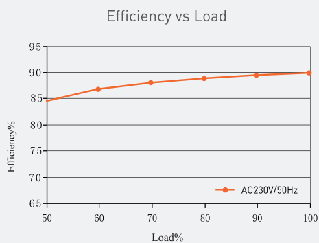
SLIM-12V-250W
